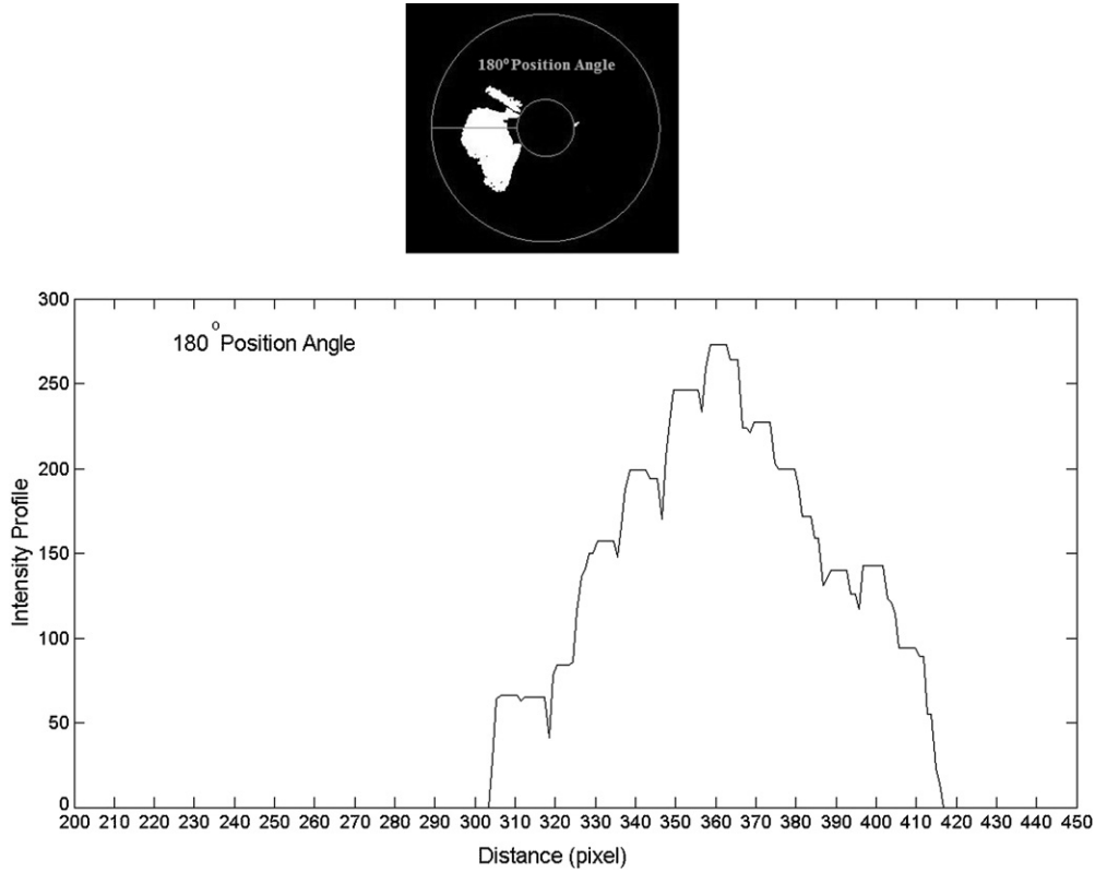
Figure 2. Example of the projection intensity profile to 180° position angle (top). Our chosen field of view is represented by the gray circles in the top panel. The bottom panel shows the 2D images intensity profile, along the 180° angular axis, as a function of distance (in pixel values). CME in a running-difference image appears as a bright leading-edge enhancement (positive pixel values).
